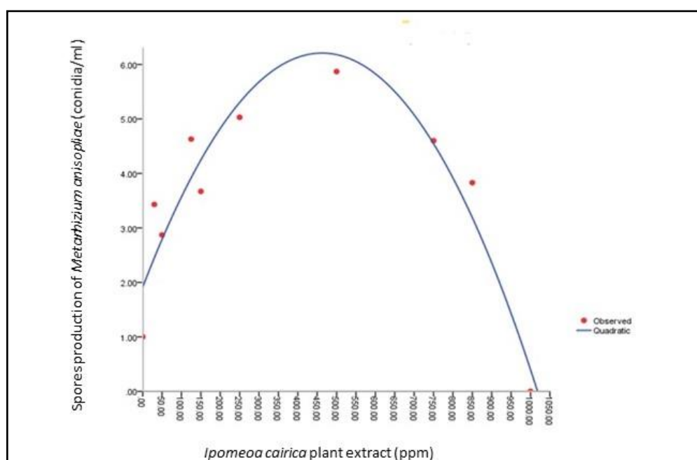
Figure 1. The curves estimation regression between Metarhizium anisopliae and Ipomeoa cairica
